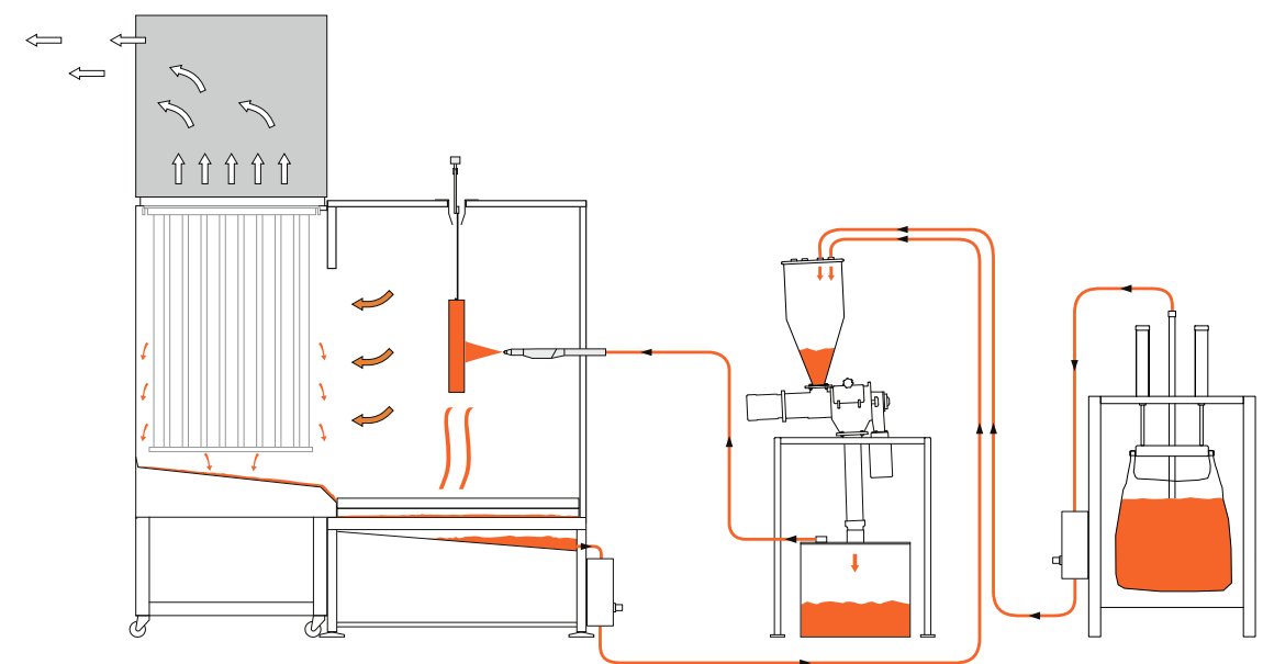
Closed and efficient powder circuit of MRS booth - single-color application
